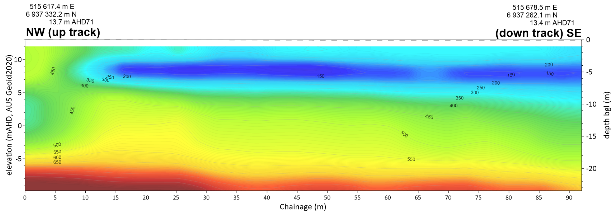
Seismic Line MASW AU-GP 162-2 P1
